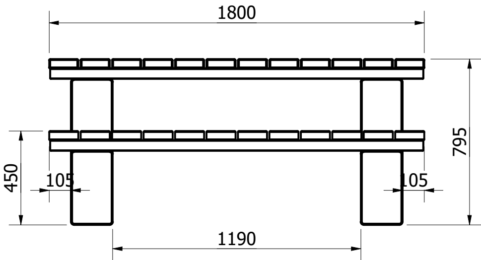
FRONT VIEW ( 1 : 18 )
