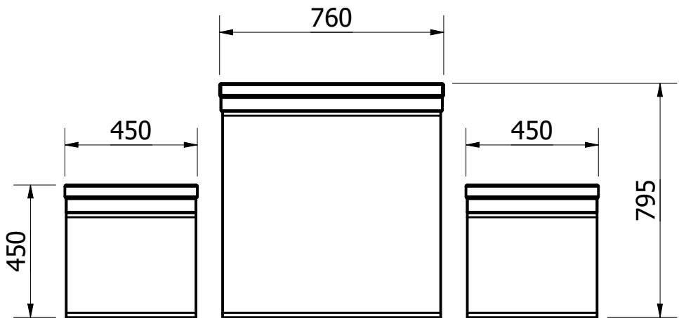
SIDE VIEW ( 1 : 18 )
