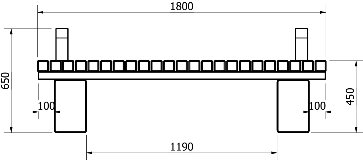
FRONT VIEW ( 1 : 14 )
