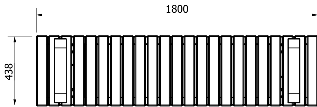
TOP VIEW ( 1 : 14 )
