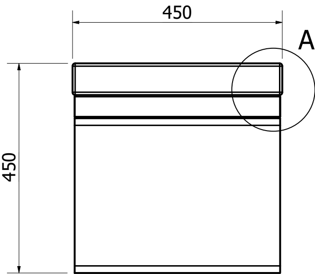
SIDE VIEW ( 1 : 8 )
