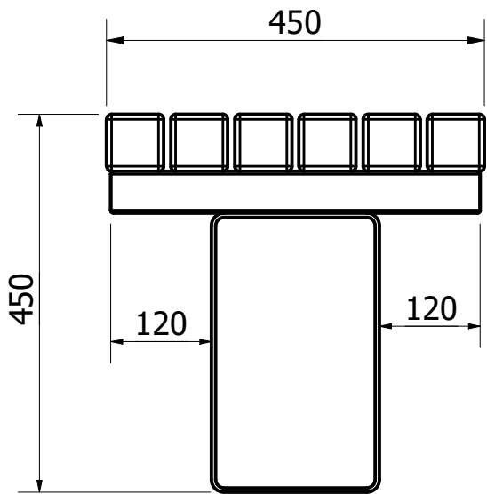
FRONT VIEW ( 1 : 8 )
