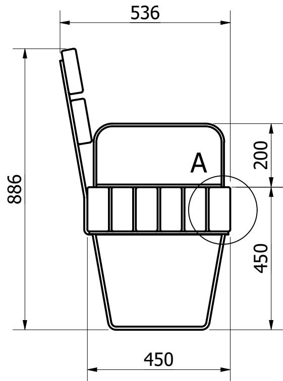
SIDE VIEW ( 1 : 12 )
