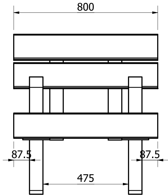
FRONT VIEW ( 1 : 12 )
