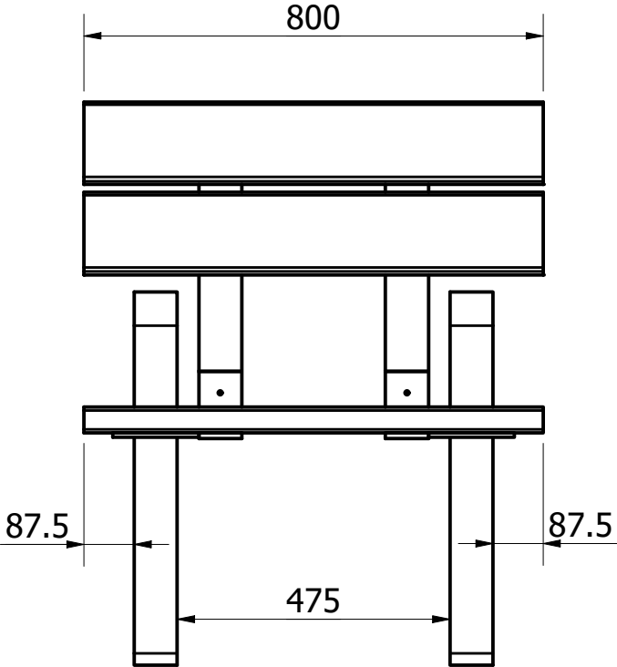
FRONT VIEW ( 1 : 12 )
