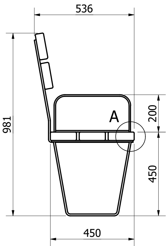
SIDE VIEW ( 1 : 12 )
