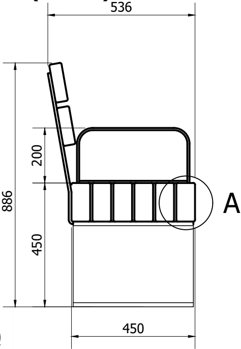
SIDE VIEW ( 1 : 14 )
