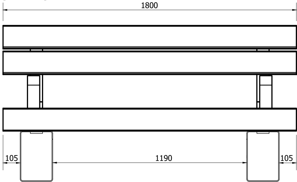
FRONT VIEW ( 1 : 14 )
