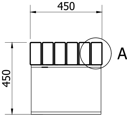
SIDE VIEW ( 1 : 14 )
