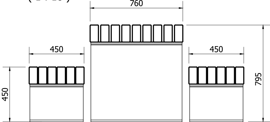
SIDE VIEW ( 1 : 18 )
