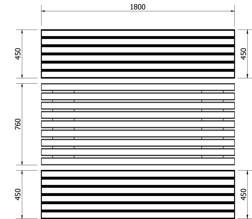
TOP VIEW ( 1 : 18 )
