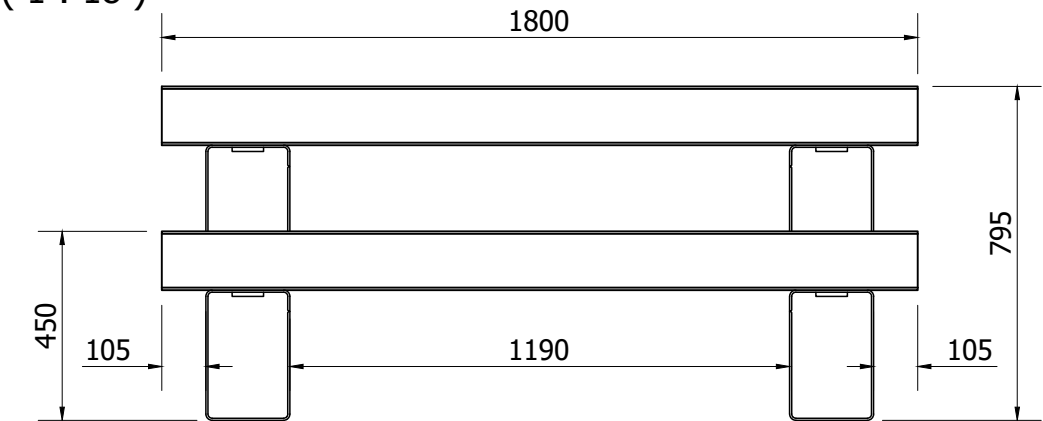
FRONT VIEW ( 1 : 18 )
