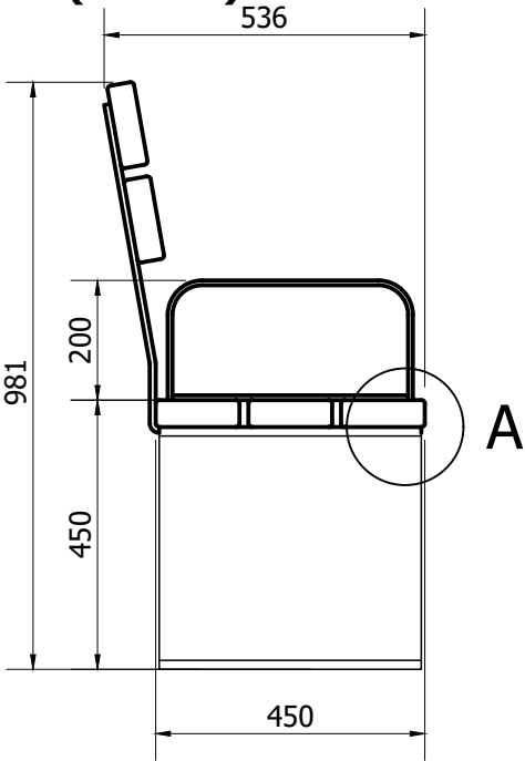
SIDE VIEW ( 1 : 14 )
