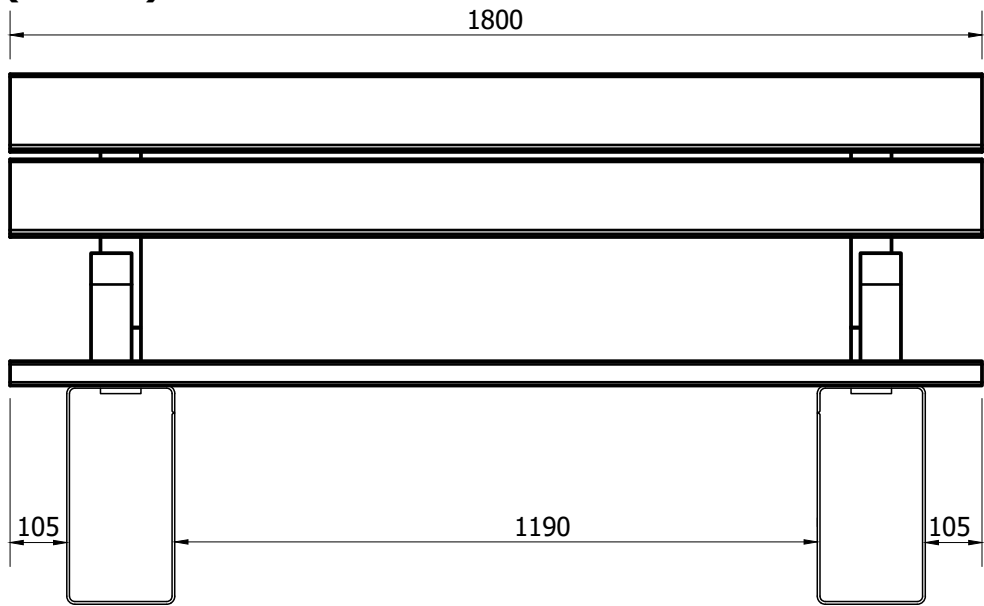
FRONT VIEW ( 1 : 14 )
