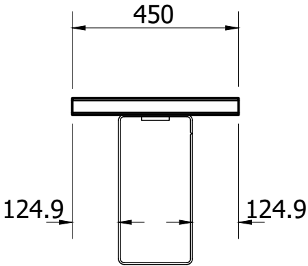
FRONT VIEW ( 1 : 14 )
