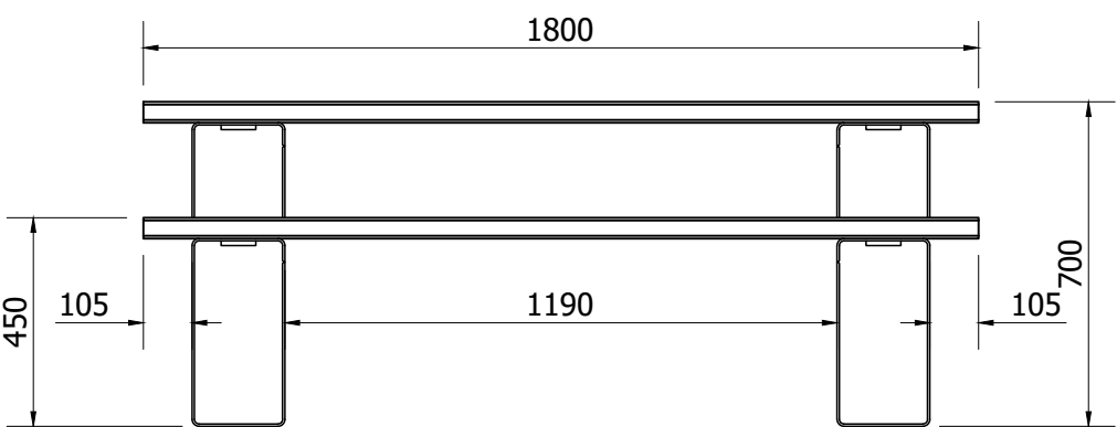
FRONT VIEW ( 1 : 18 )
