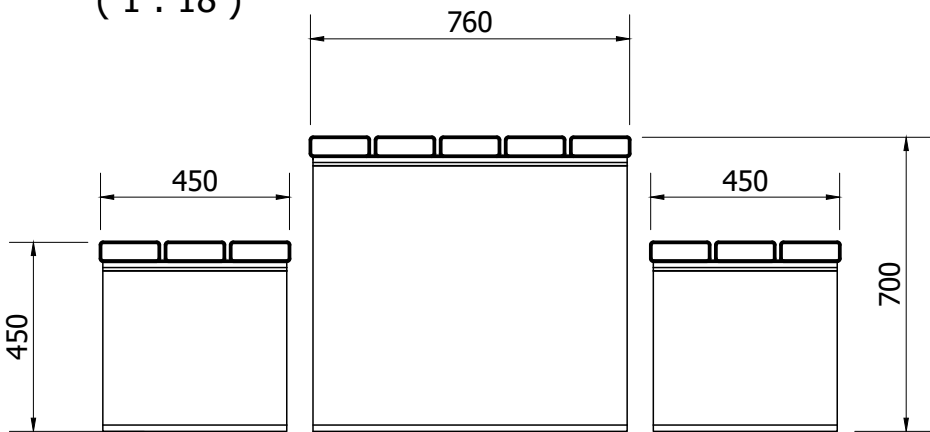
SIDE VIEW ( 1 : 18 )
