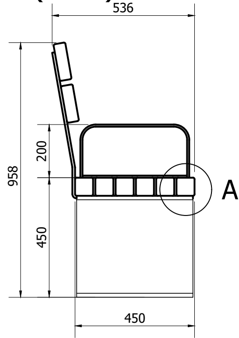
SIDE VIEW ( 1 : 14 )
