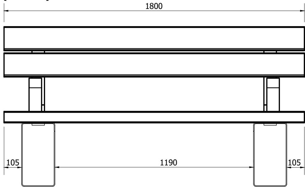
FRONT VIEW ( 1 : 14 )
