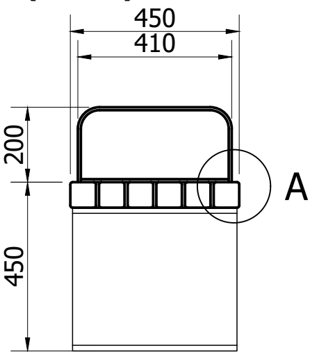
SIDE VIEW ( 1 : 14 )
