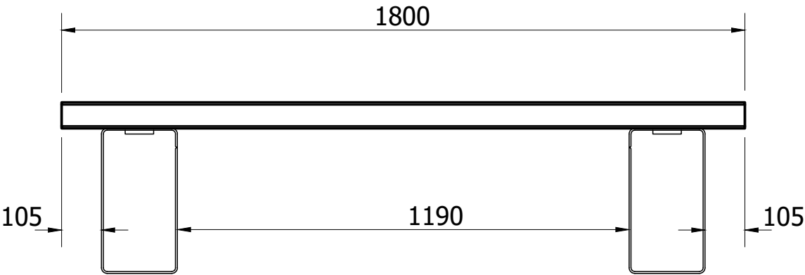
FRONT VIEW ( 1 : 14 )
