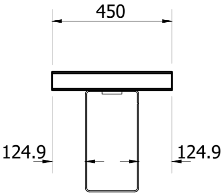
FRONT VIEW ( 1 : 14 )
