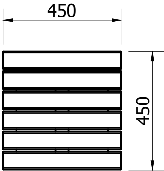
TOP VIEW ( 1 : 14 )
