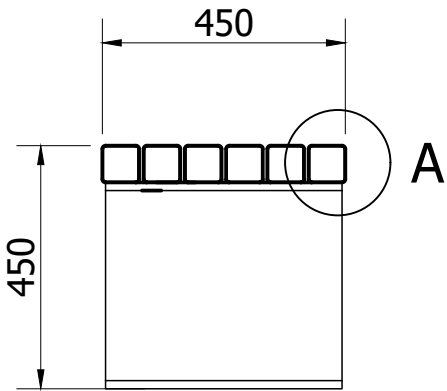
SIDE VIEW ( 1 : 14 )
