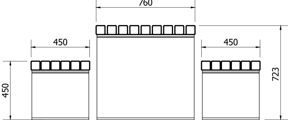
SIDE VIEW ( 1 : 18 )
