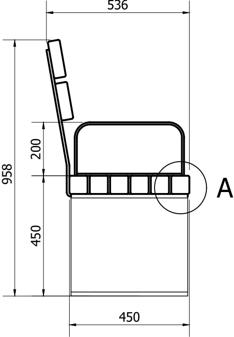
SIDE VIEW ( 1 : 14 )
