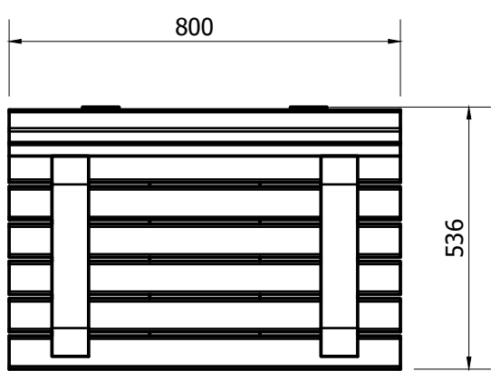
TOP VIEW ( 1 : 14 )
